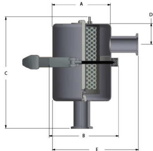
VTL Configuration
