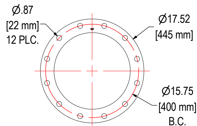
DETAIL A DN300 FLANGE BOLT PATTERN
