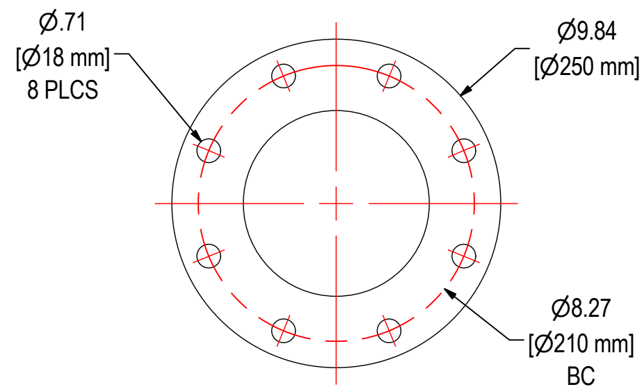
DETAIL A DN125/PN10 FLANGE BOLT PATTERN
