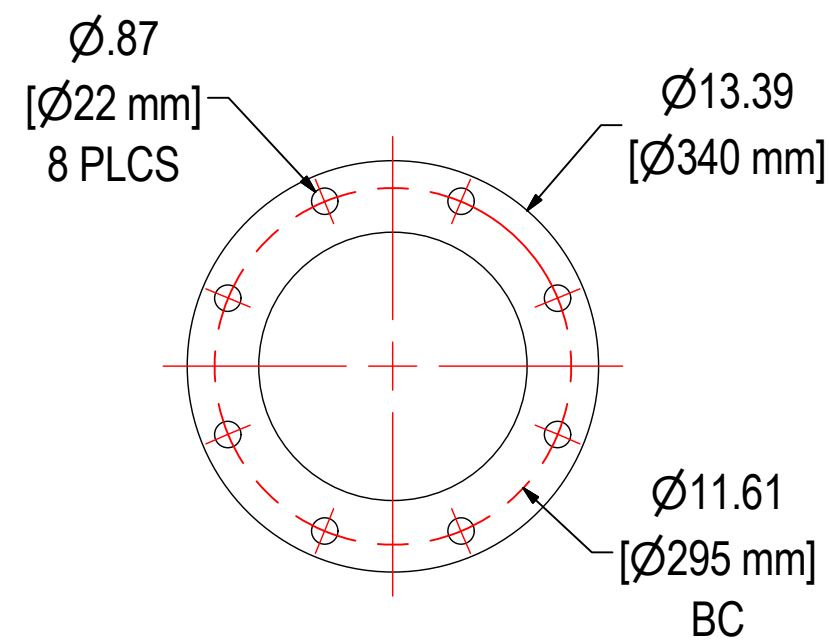
DETAIL A SCALE 0.16 : 1 DN200/PN10 FLANGE BOLT PATTERN
