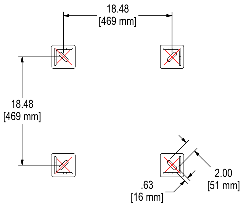
FOOTPAD LAYOUT
