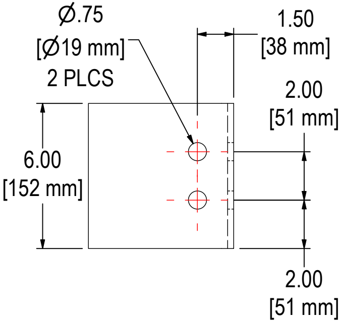
MOUNTING BRACKET
